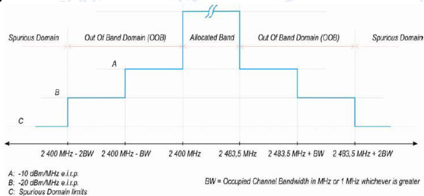
Figure 1: Transmit mask
